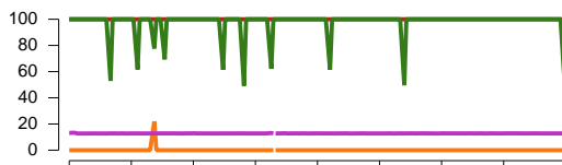
CSI-Windows-Sharepoint-BPWSSWZWD01
